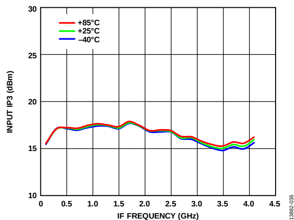
Figure 36. Input IP3 vs. IF Frequency at Various Temperatures, LO = 15 dBm
