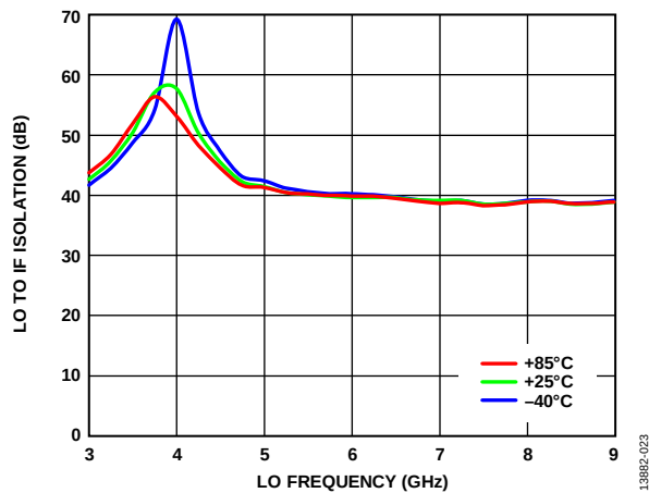
Figure 23. LO to IF Isolation vs. LO Frequency at Various Temperatures, LO = 15 dBm
