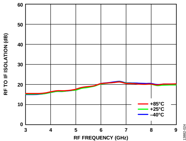
Figure 24. RF to IF Isolation vs. RF Frequency at Various Temperatures, LO = 15 dBm
