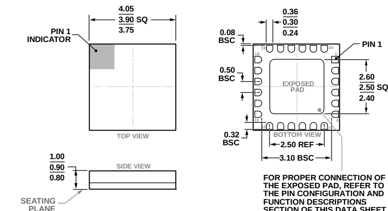
Figure 41. 24-Terminal Ceramic Leadless Chip Carrier (LCC) (E-24-1) Dimensions shown in millimeters
