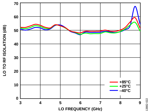
Figure 22. LO to RF Isolation vs. LO Frequency at Various Temperatures, LO = 15 dBm
