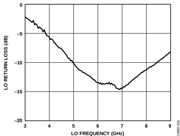
Figure 28. LO Return Loss vs. LO Frequency at 25°C, LO = 15 dBm
